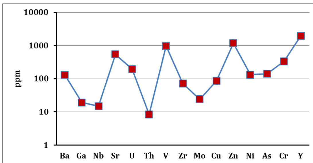
Fig.4: Profile - line diagram showing the average concentrations of the most important trace elements in the ferruginous siltstones.
