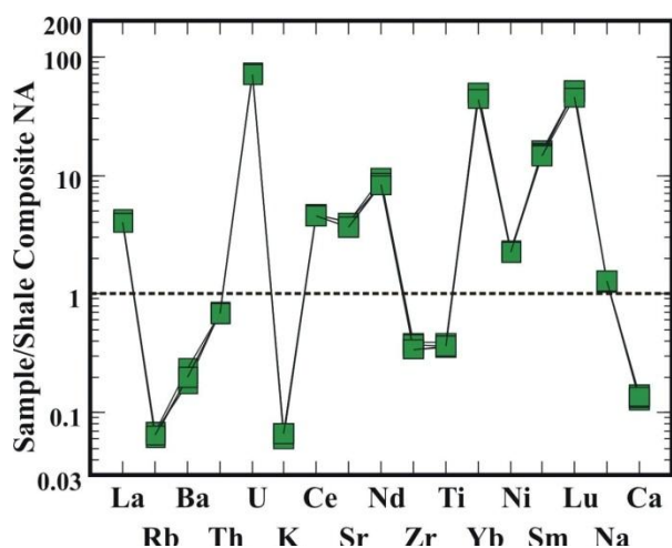
Fig.6: Trace elements pattern normalized to NASC. (Gormet et al., 1984).
