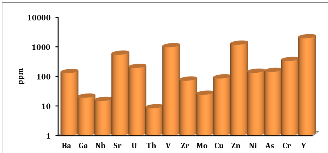
Fig.5: Bar-diagram showing the average concentrations of the most important trace elements in the ferruginous siltstones.
