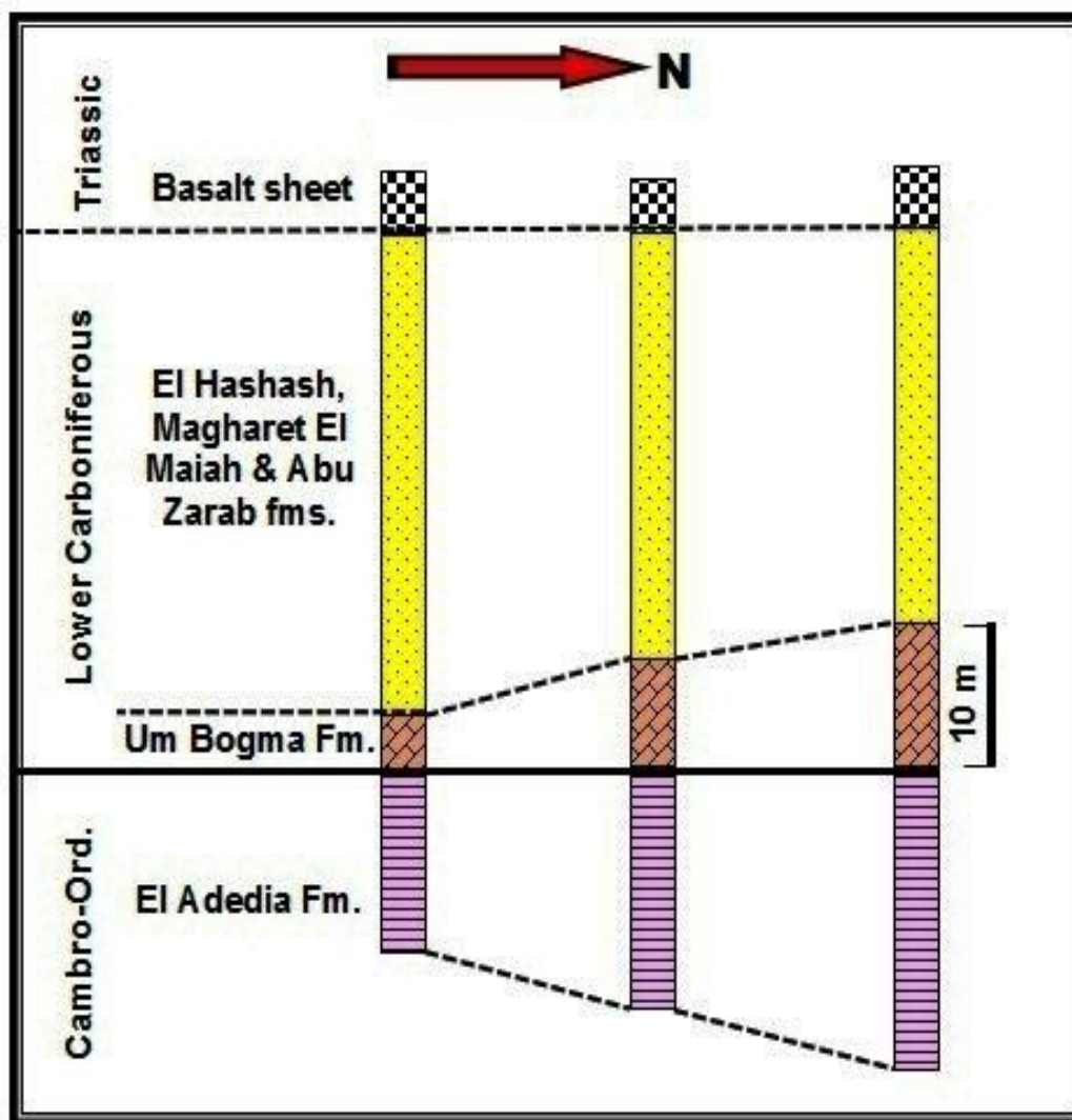
Fig. 3: Lithostratigraphic correlation along Wadi El Seih area.
