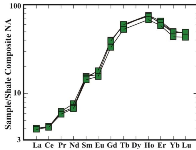
Fig. 8: Rare earth elements pattern normalized to NASC (Haskin et al., 1968).
