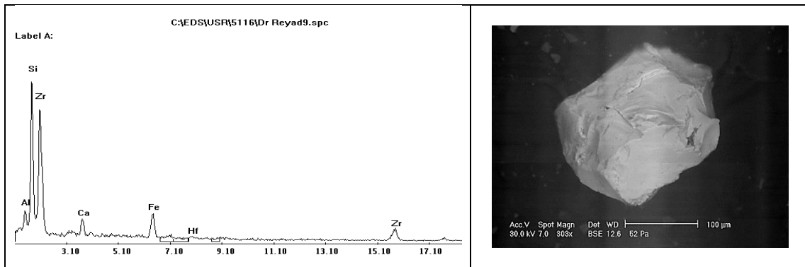
Fig. 14: EDX data and BSE image of zircon mineral.
