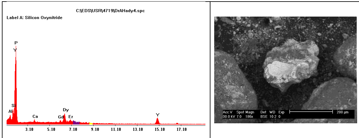
Fig. 13: EDX data and BSE image of xenotime mineral.
