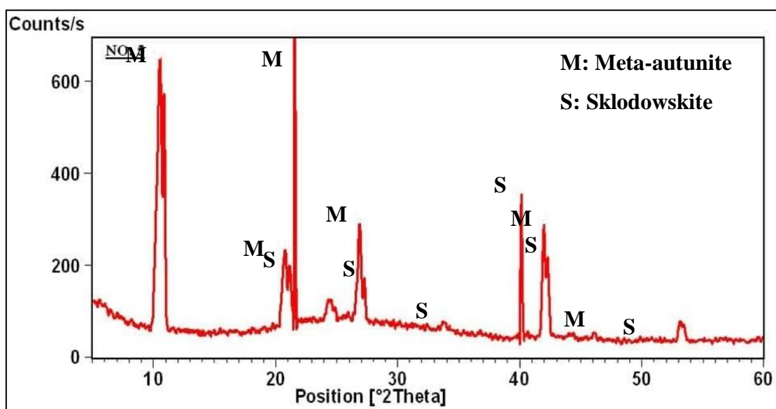
Fig. 12: XRD pattern of Meta-autunite and Sklodowskite minerals.
