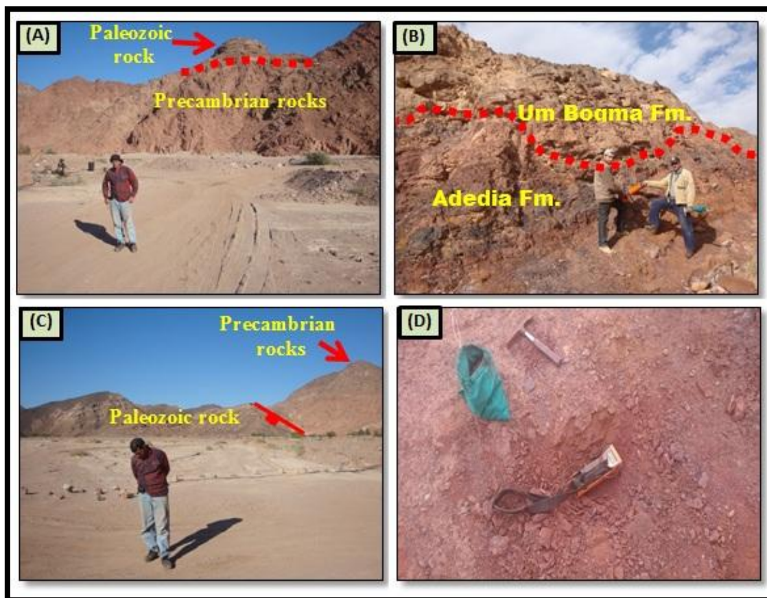
Fig. 2: (A) Precambrian rocks nonconformably overlain by Paleozoic rocks. (B) Um Bogma Formation unconformably overlies Adedia Formation. (C) Normal fault. (D) Radioactive ferruginous siltstones in the lower member of Um Bogma Formation.
