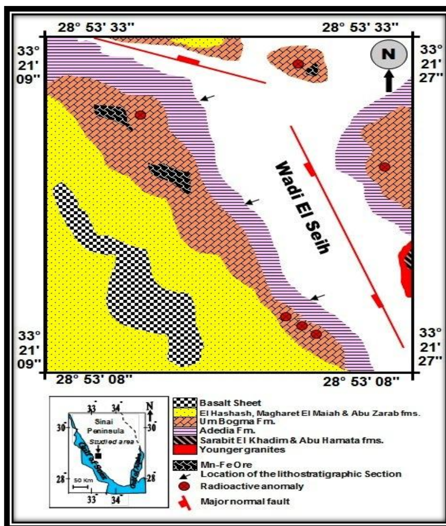
Fig. 1: Geological map of Wadi El Seih area.
