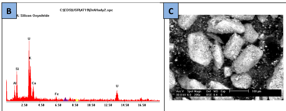
Fig. 11: XRD pattern (A), EDX data (B) and BSE image (C) of uranophane mineral.
