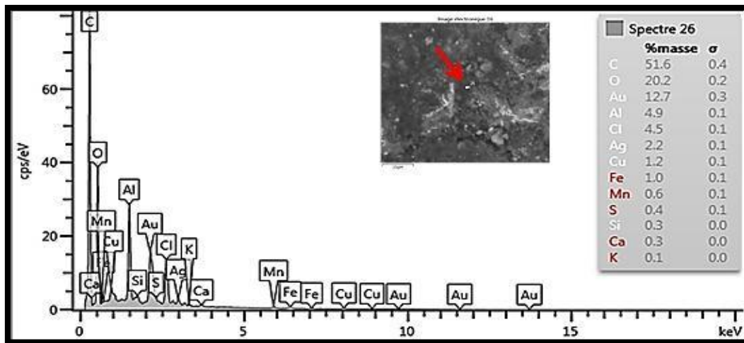
Fig. 15: EDX data and BSE image showing gold with traces of Cu, Fe and Mn.
