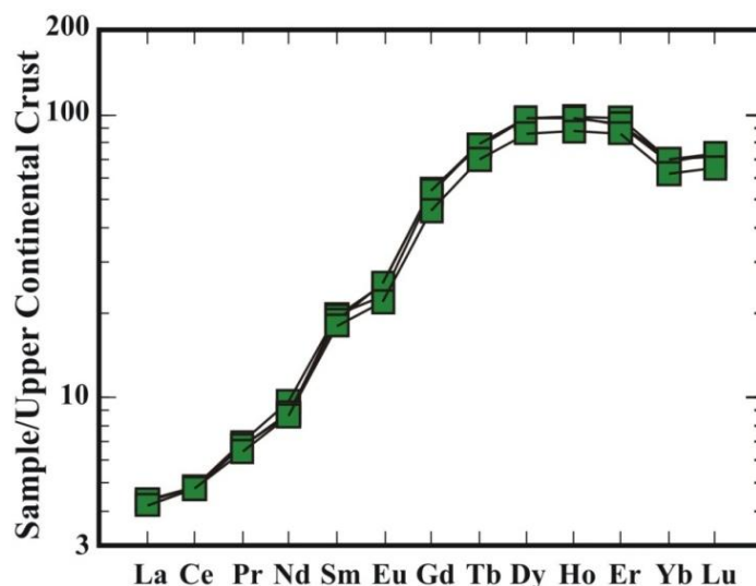
Fig. 10: REEs pattern for the studied siltstones normalized to the Upper Continental Crust (Taylor and McLennan, 1981).
