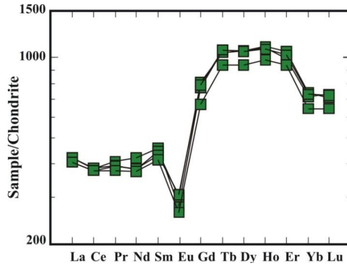
Fig. 7: Rare earth element elements pattern of the studied siltstones normalized to Chondrite (Boynton, 1984).
