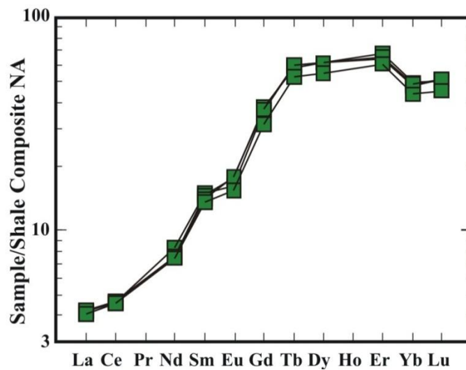
Fig. 9: Rare earth elements pattern normalized with NASC. (Gromet et al., 1984)
